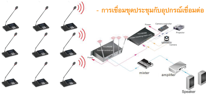
Voice Tracking Camera (YC531) Video Tracking Main Unit (YCV800M)
